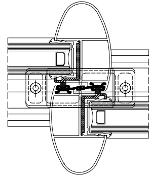
Snitt-tegning overlapping
